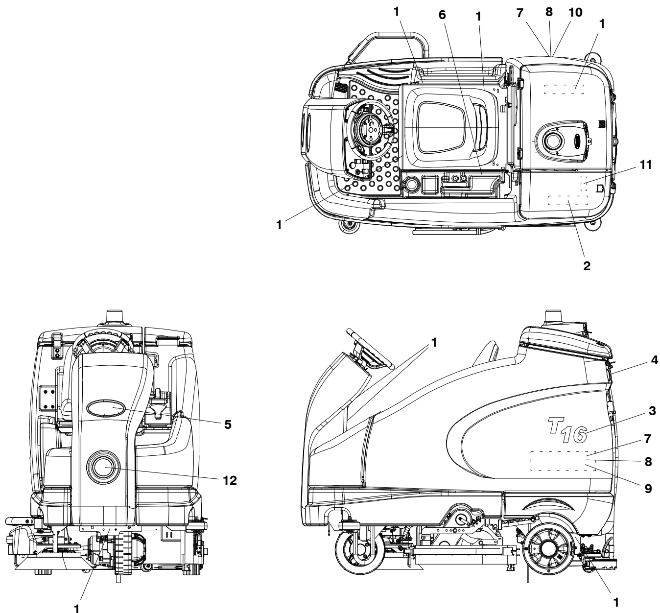
Fig. 26 – Label Group
