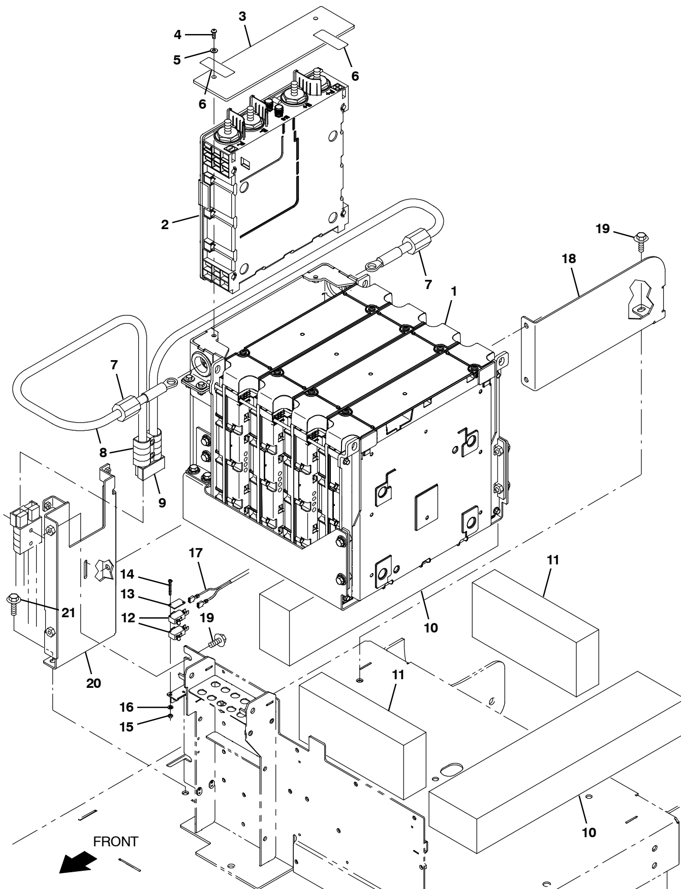
Fig. 38 - Battery Group, Lithium-Ion, 36V, 8.2 Kwh
