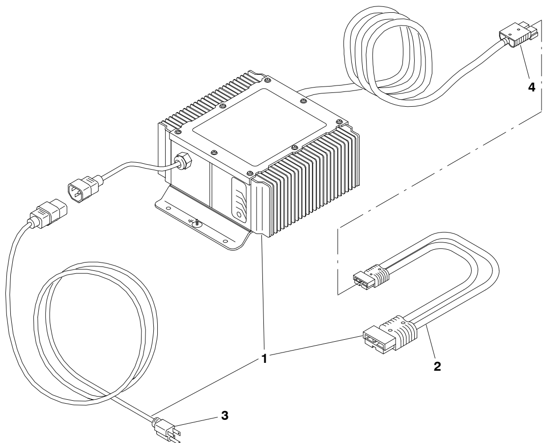
Fig. 41 – Battery Charger Group (Rollout Battery)
