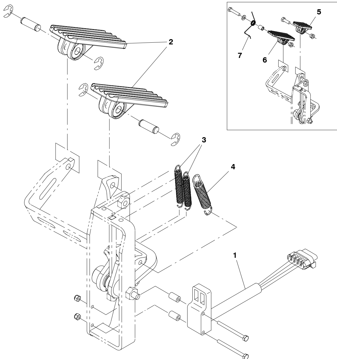
Fig. 10 – Accelerator and Brake Pedal Assembly Breakdown, 1051837
