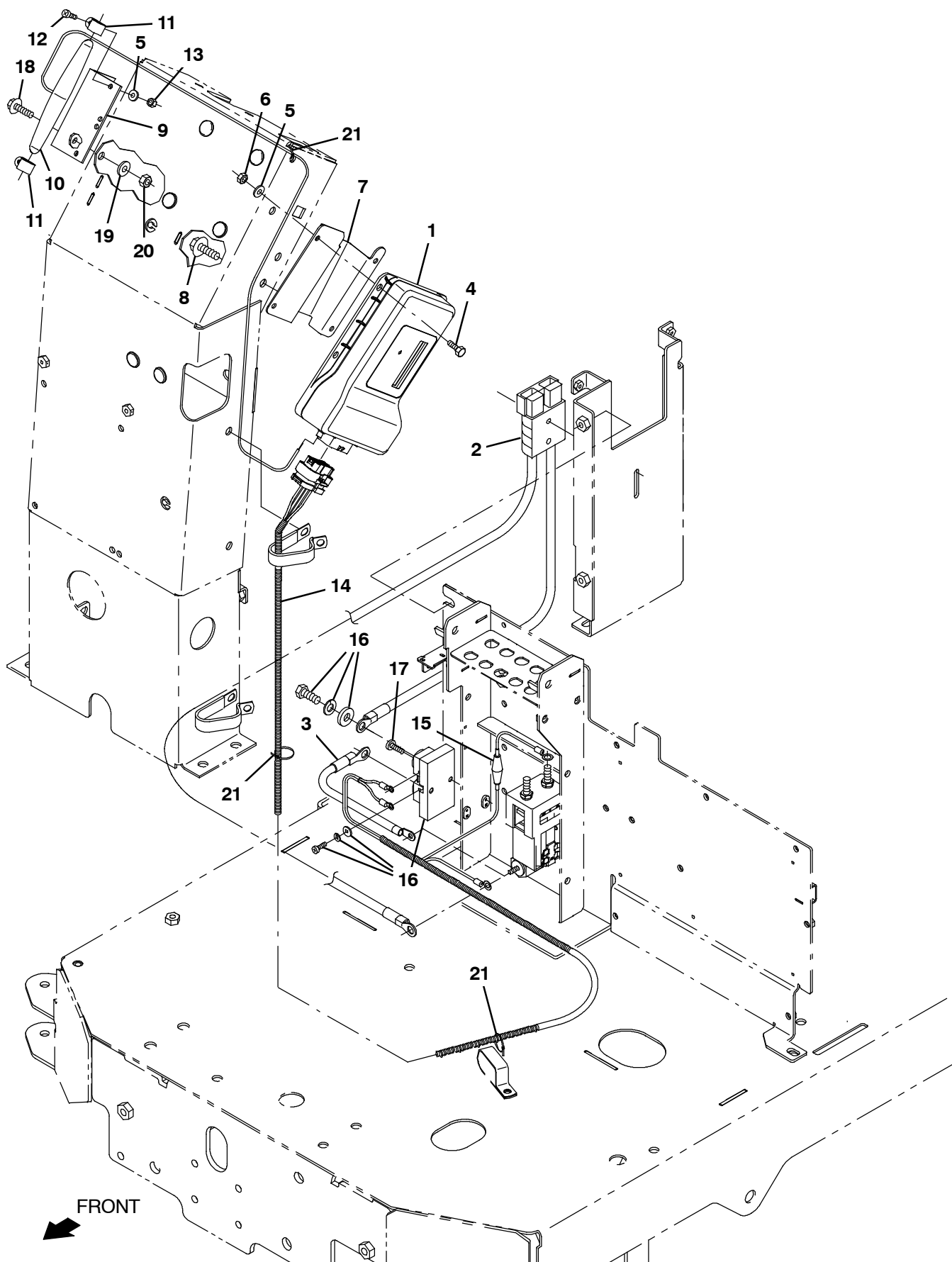
Fig. 54 - Telemetry Group
