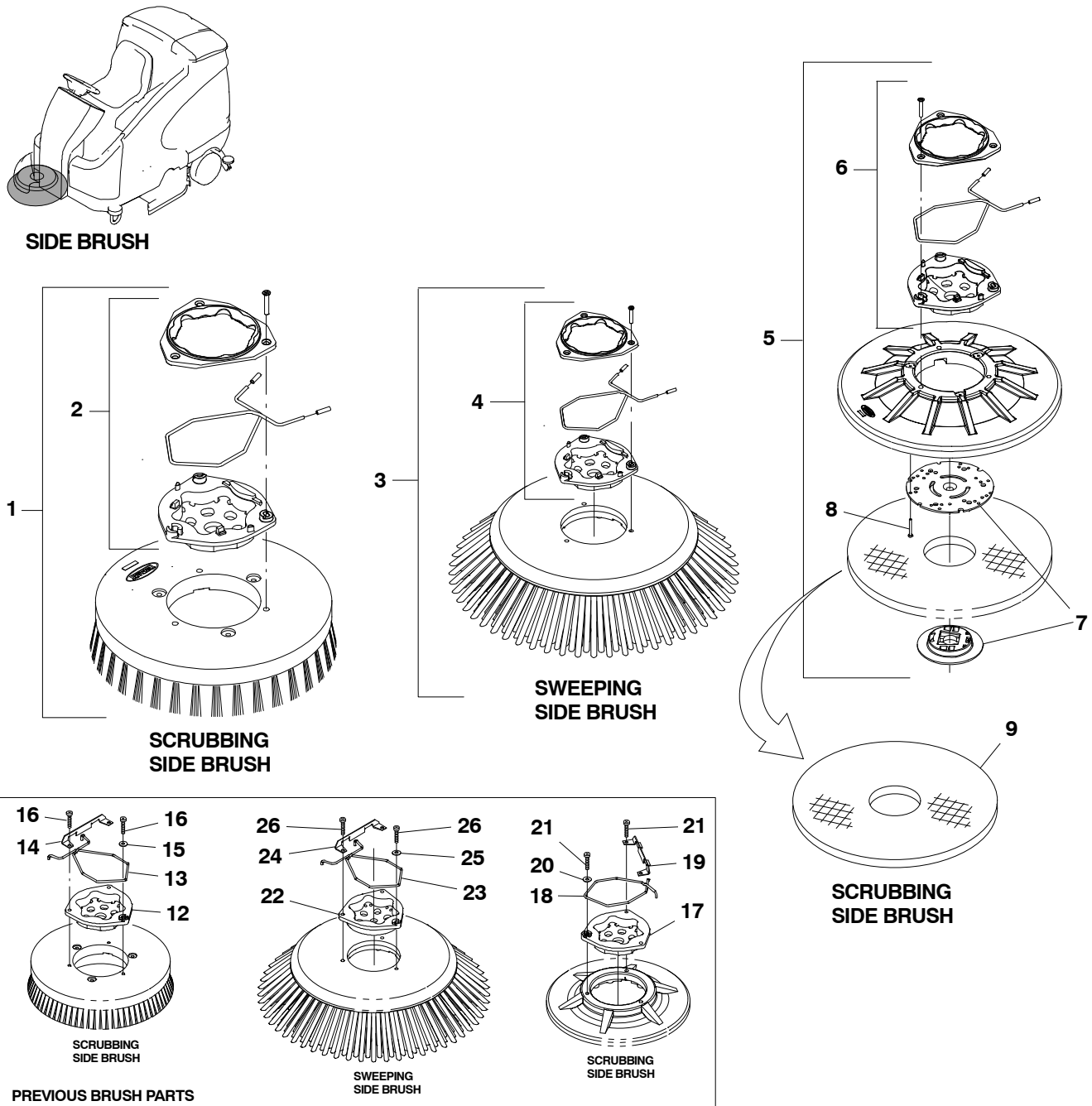
Fig. 2 – Replacement Brushes, Side Brush and Pre-Sweep
