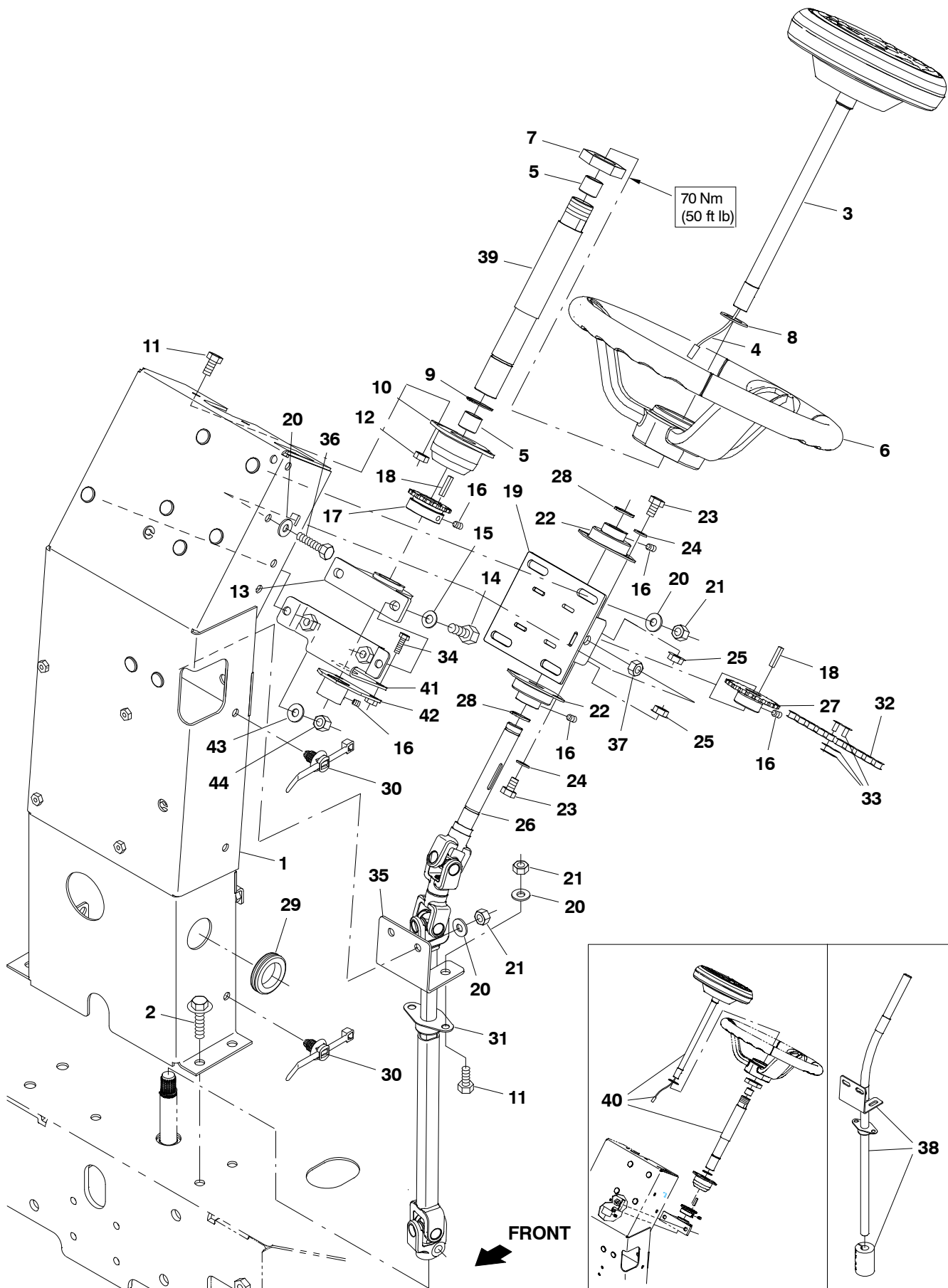
Fig. 5 – Steering Group
