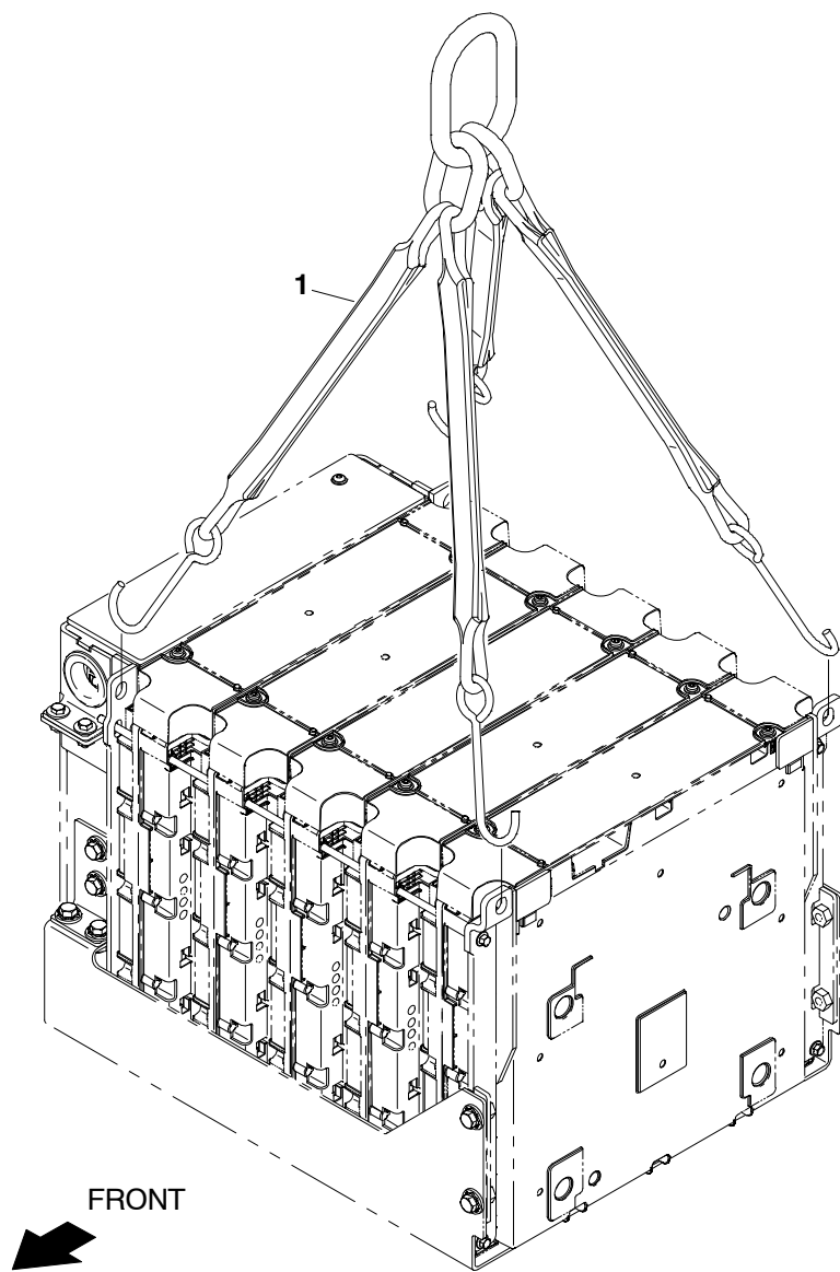
Fig. 25 – Lithium-Ion Battery Lifting Kit
