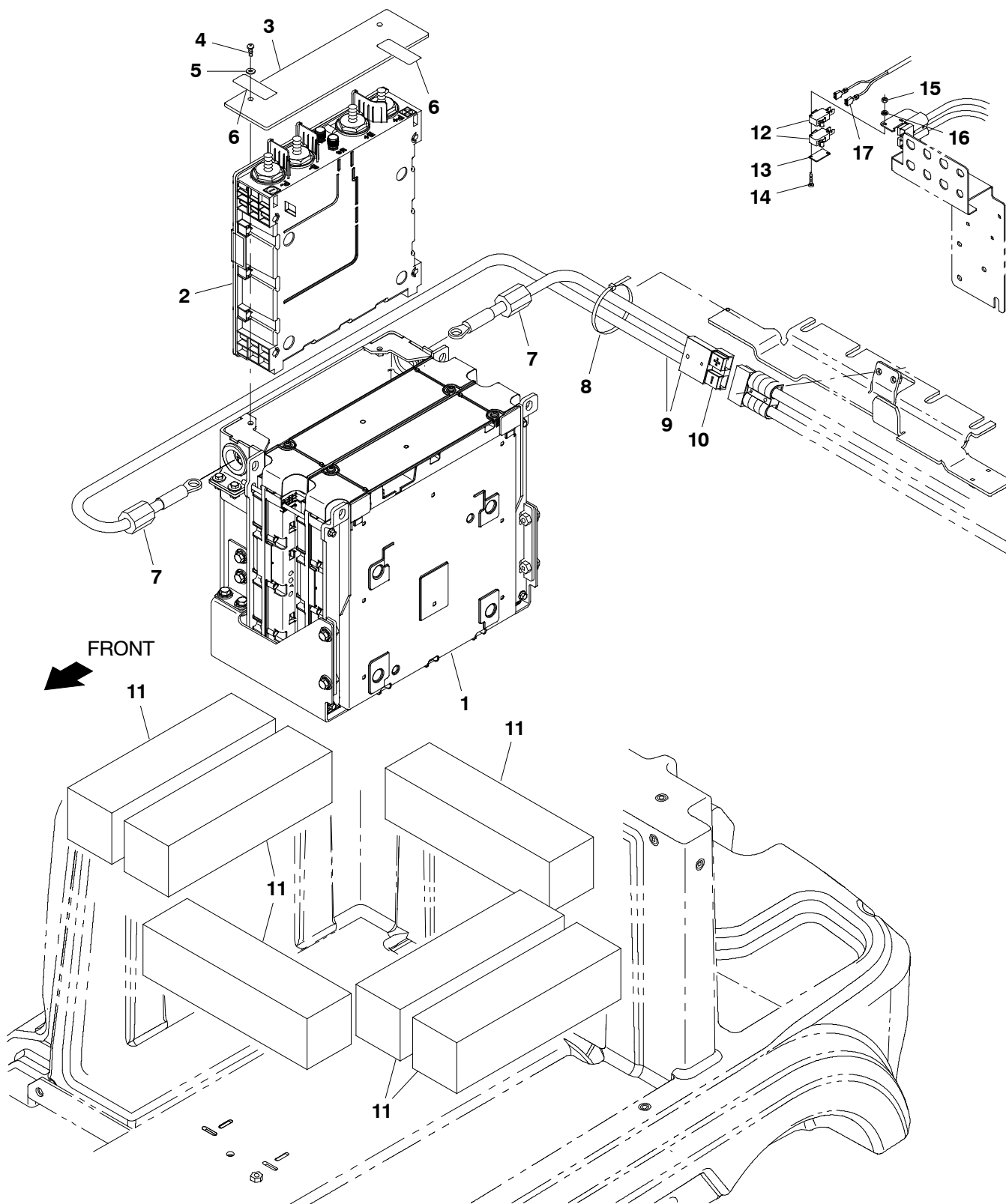
Fig. 24 - Battery Group, Lithium-Ion, 36V, 4.1 Kwh
