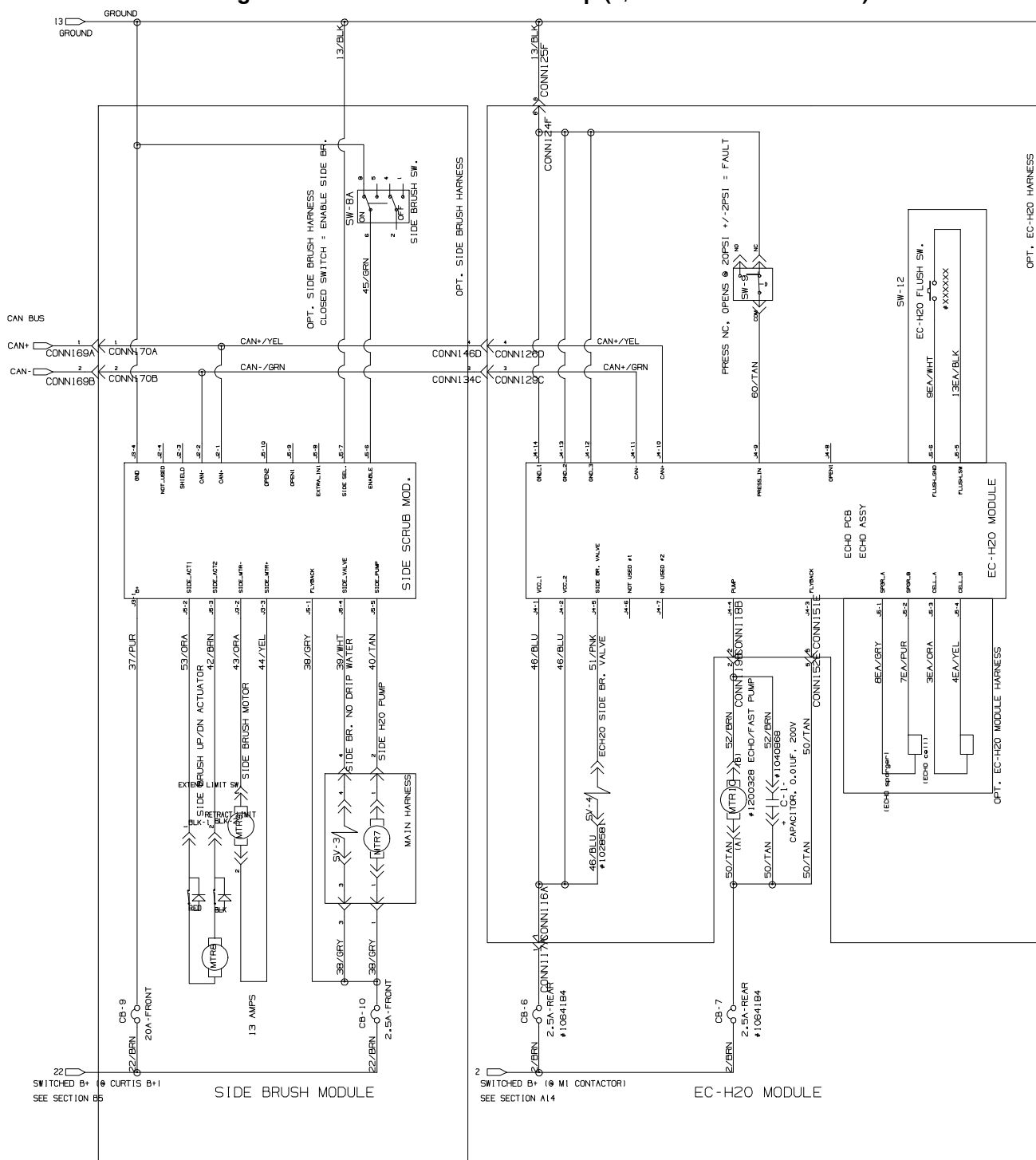
Fig. 25 – Electrical Schematic Group (S/N 1000000–10863997)
