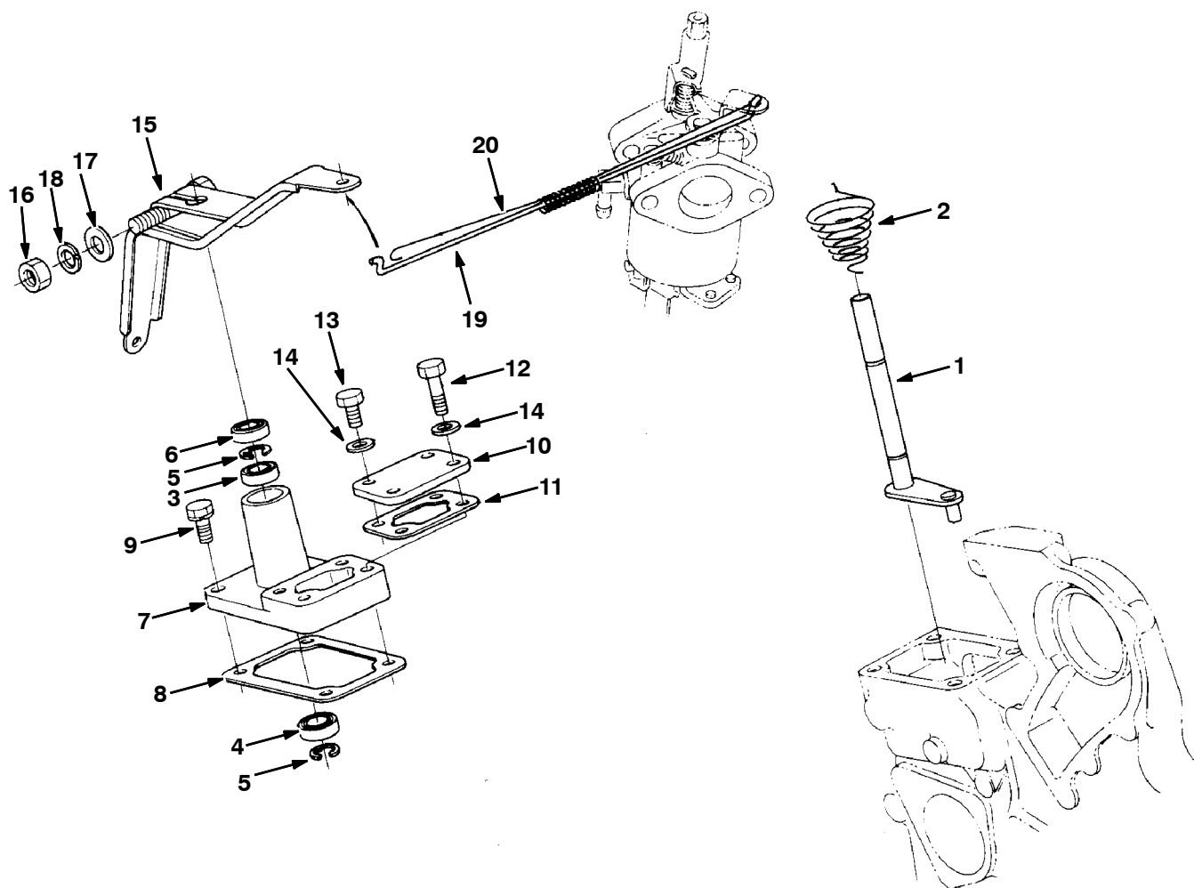
Fig. 13 - Governor Group
