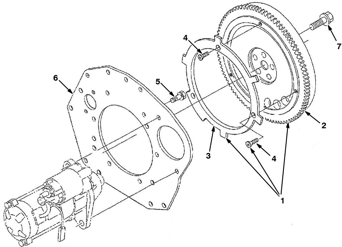
Fig. 9 - Flywheel Group
