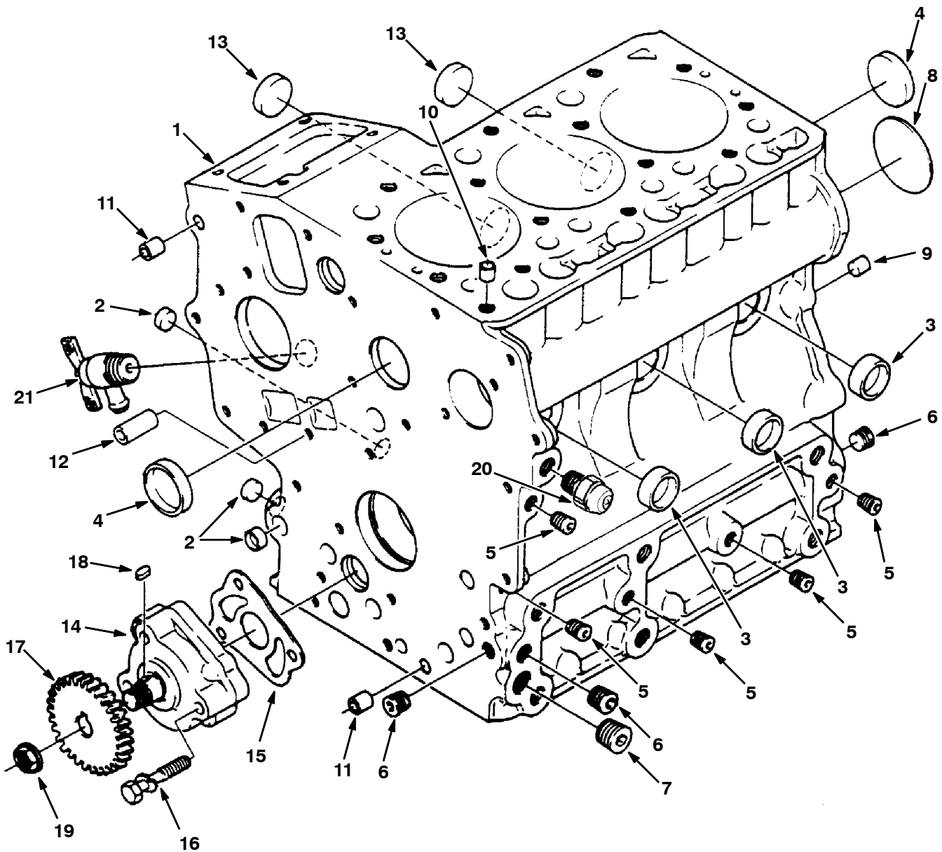
Fig. 1 - Crankcase Group
