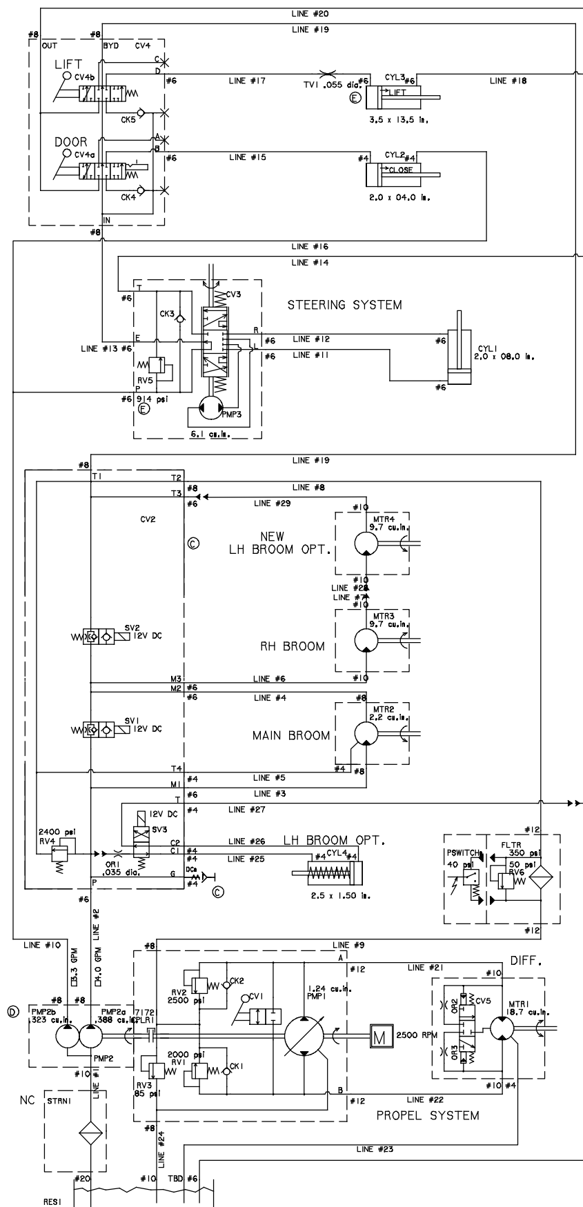
Fig. 40 - Hydraulic Schematic
