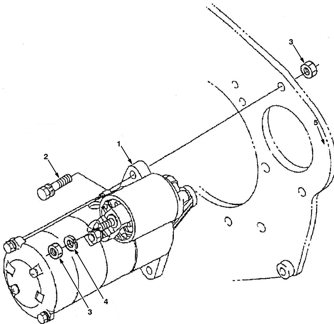
Fig. 19 - Starter Group
