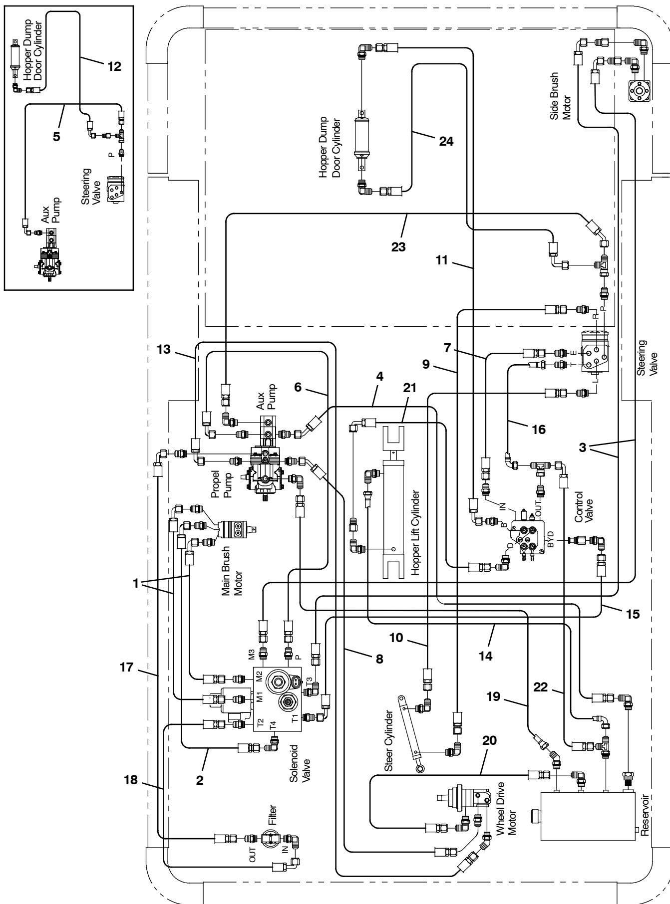
Fig. 42 - Hydraulic Hose Group (003000- )
