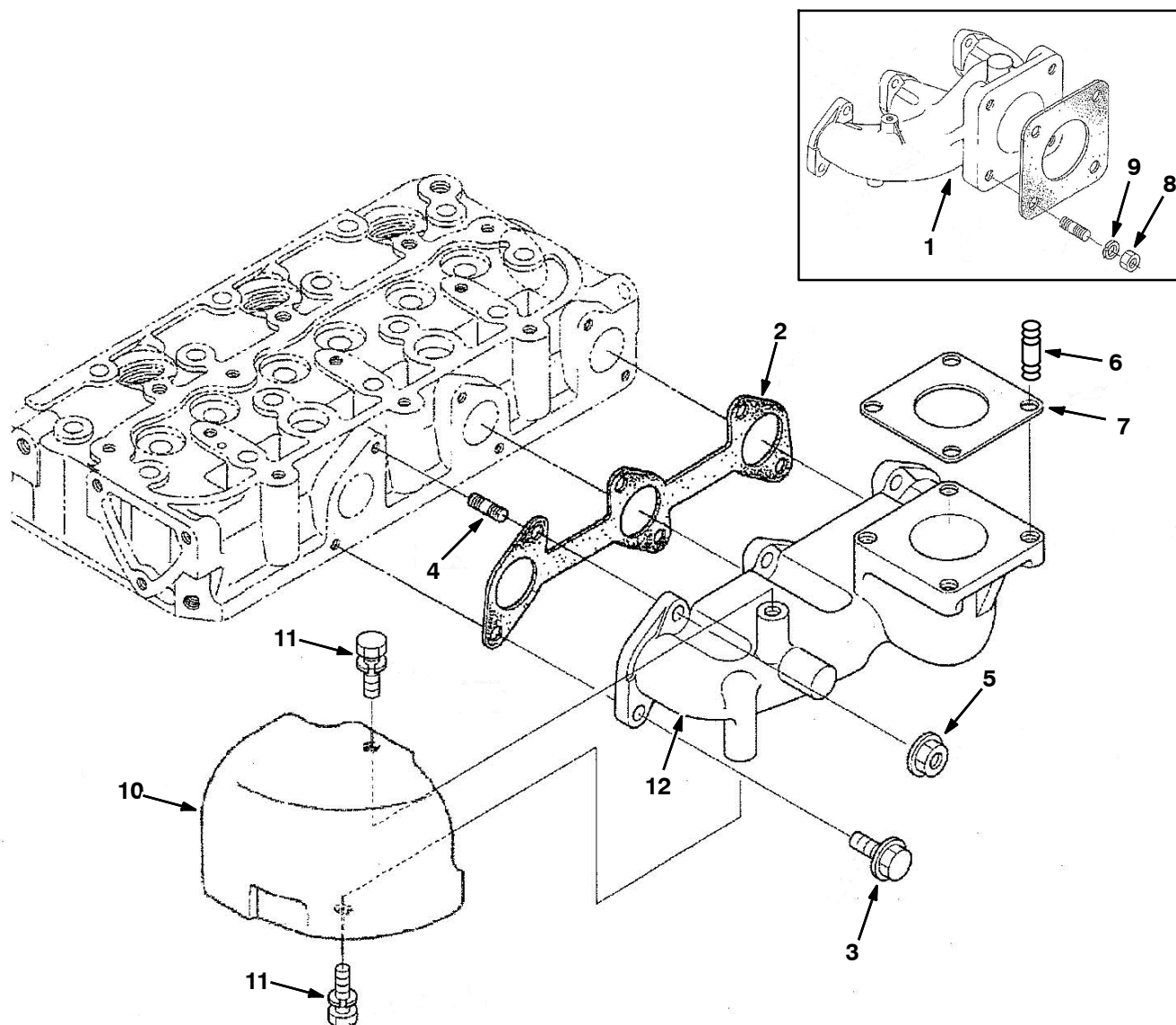
Fig. 25 - Exhaust Manifold Group
