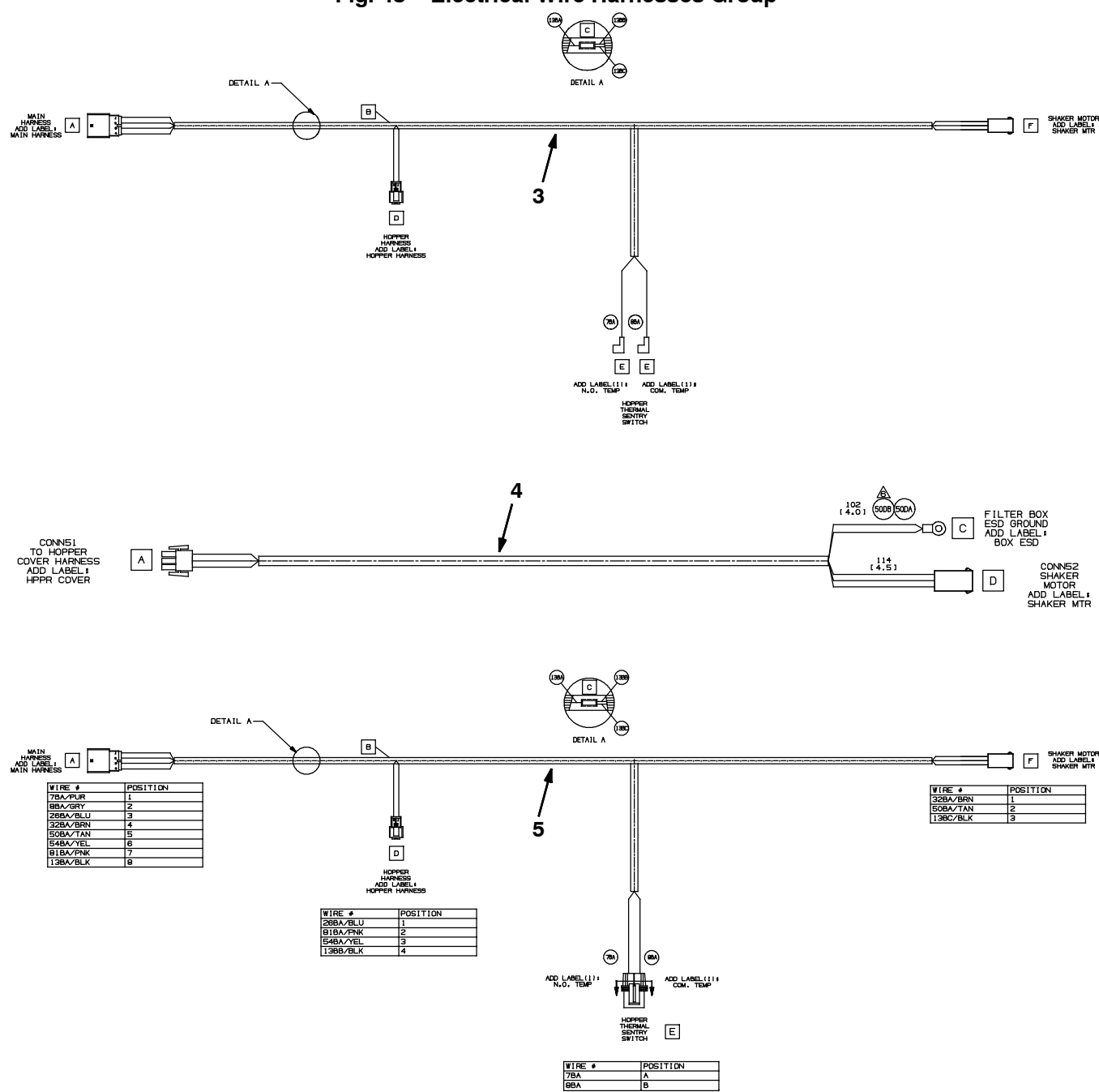
Fig. 48 - Electrical Wire Harnesses Group
