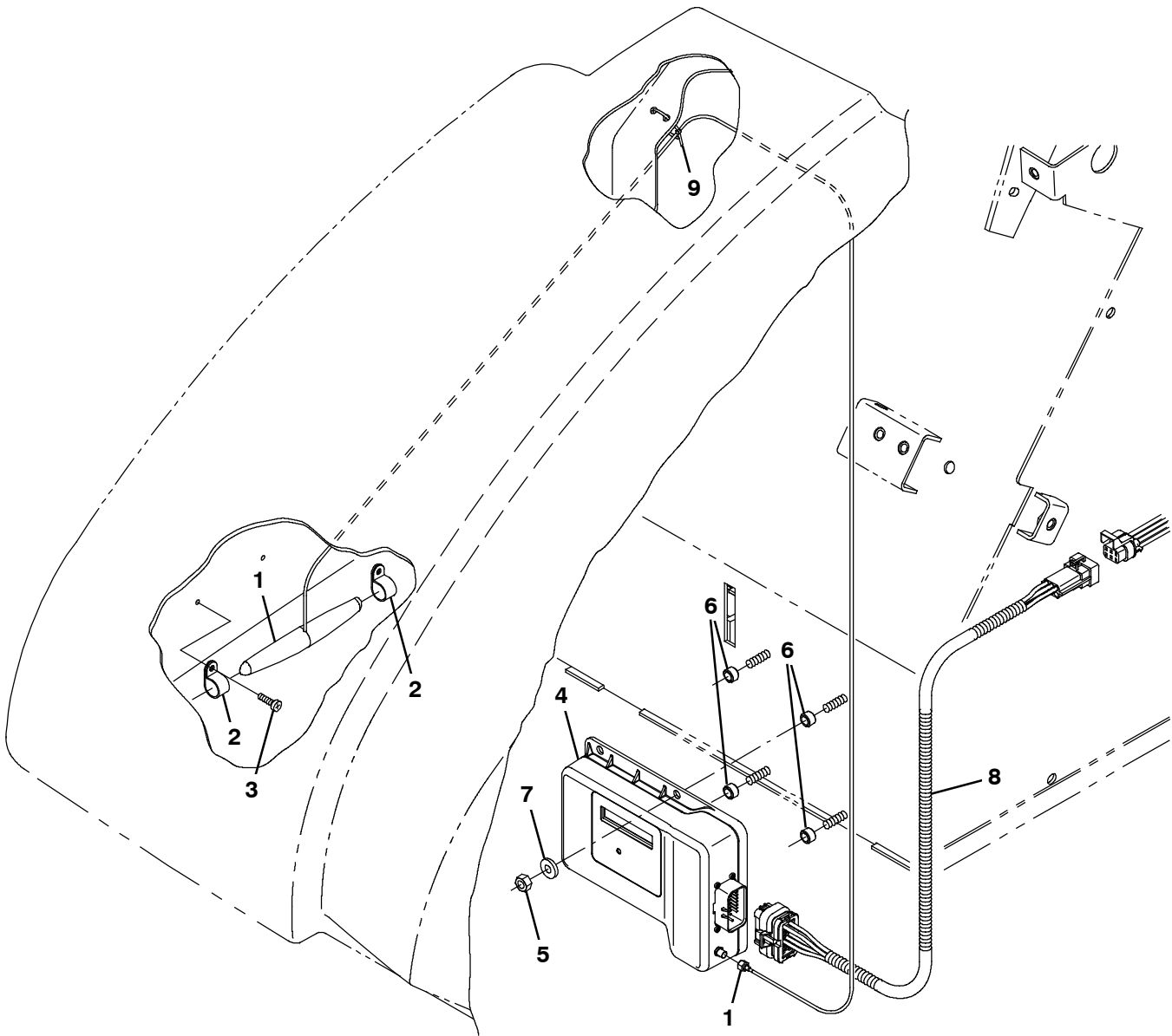
Fig. 30 - Telemetry Group
