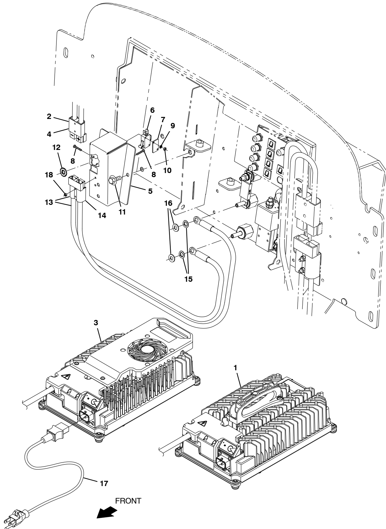
Fig. 16 – Off-Board Battery Chargers Group
