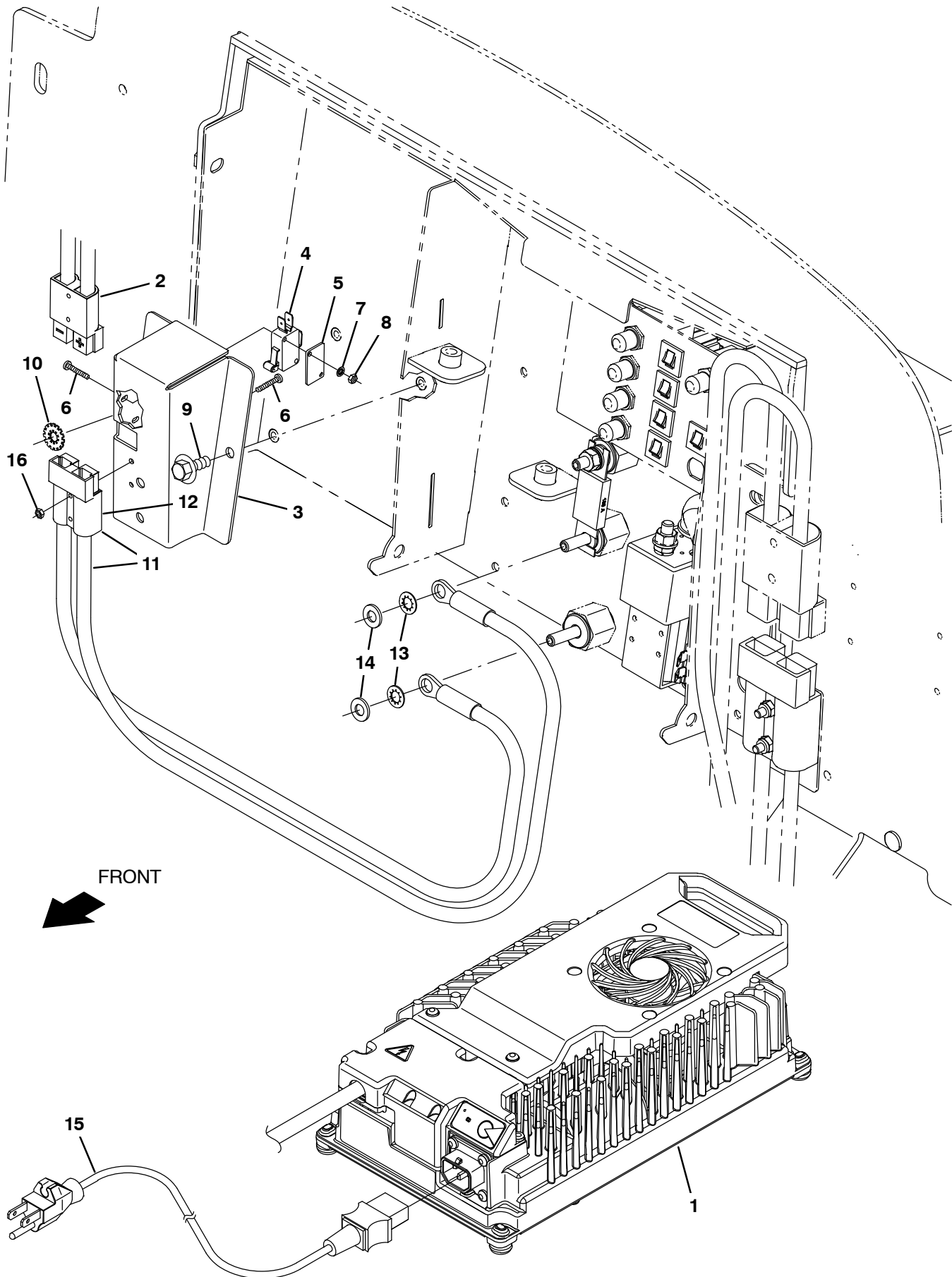
Fig. 17 – Off-Board Lithium-Ion Battery Charger Group
