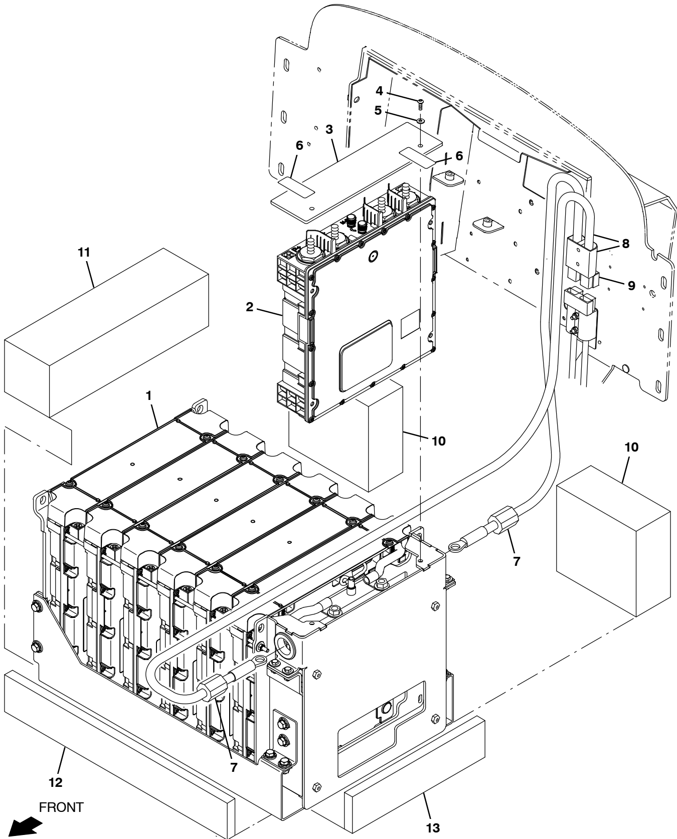
Fig. 12 – Battery Group, Lithium-Ion, 36V, 12.2 Kwh
