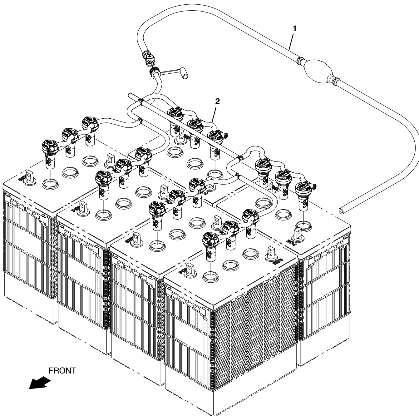
Fig. 19 – Manual Battery Watering System
