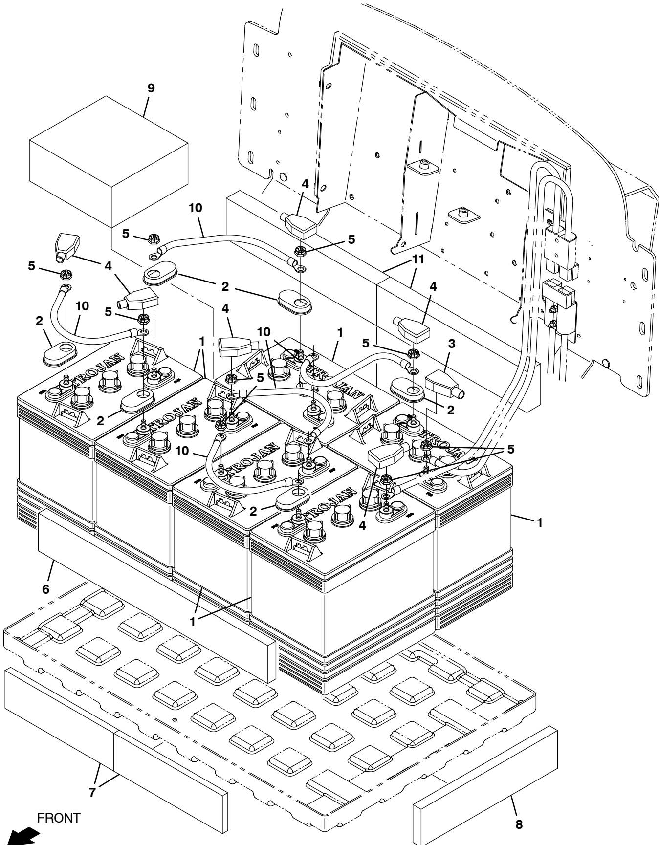
Fig. 11 – Battery Group, Wet, 36V 240Ah
