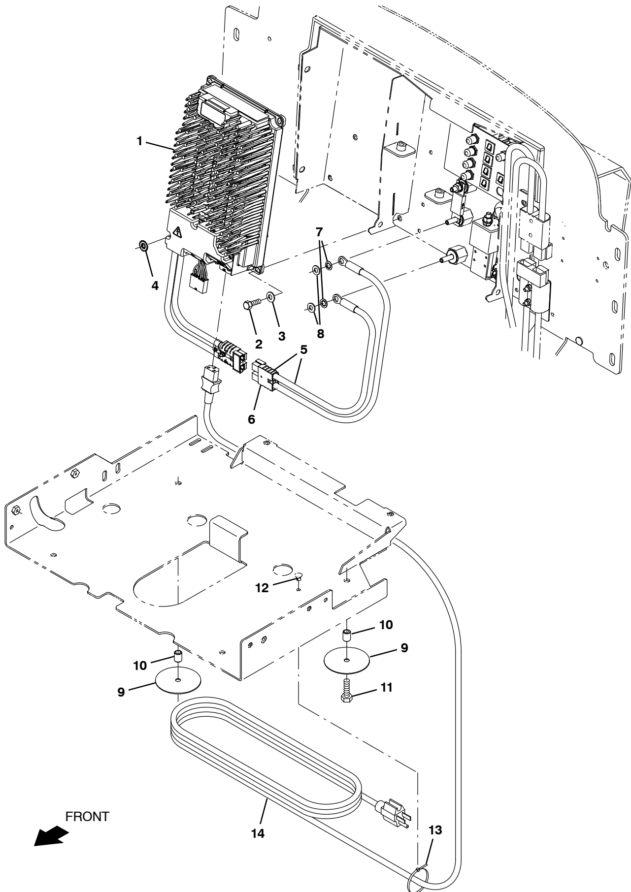
Fig. 15 – On-Board Battery Charger Group
