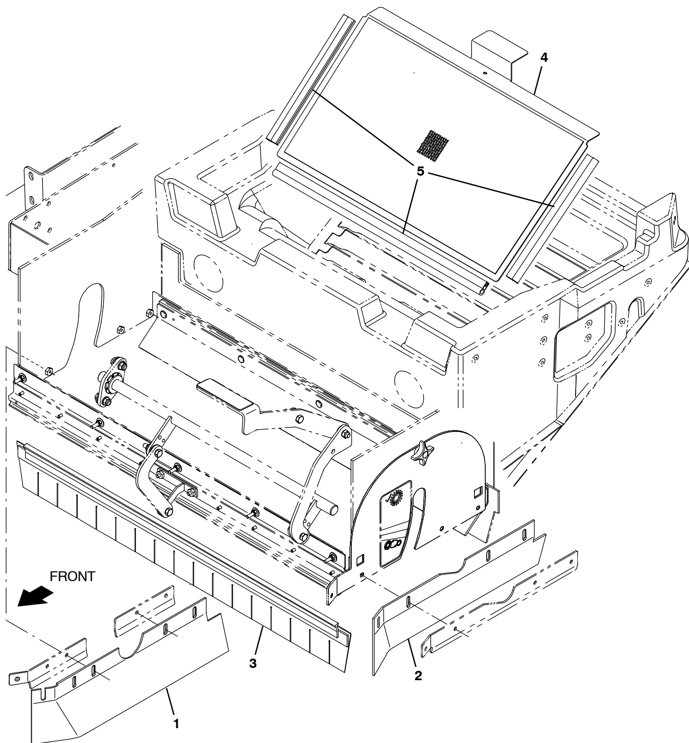
Fig. 20 – Carpet Care Kit
