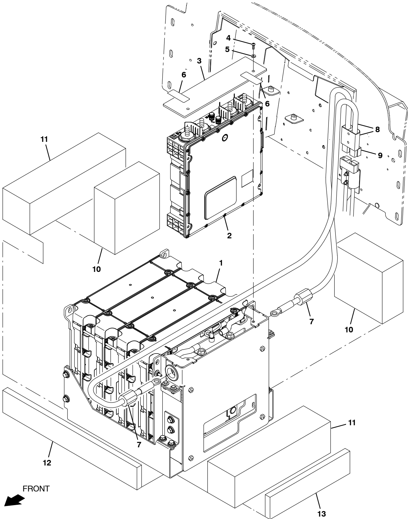
Fig. 13 – Battery Group, Lithium-Ion, 36V, 8.2 Kwh
