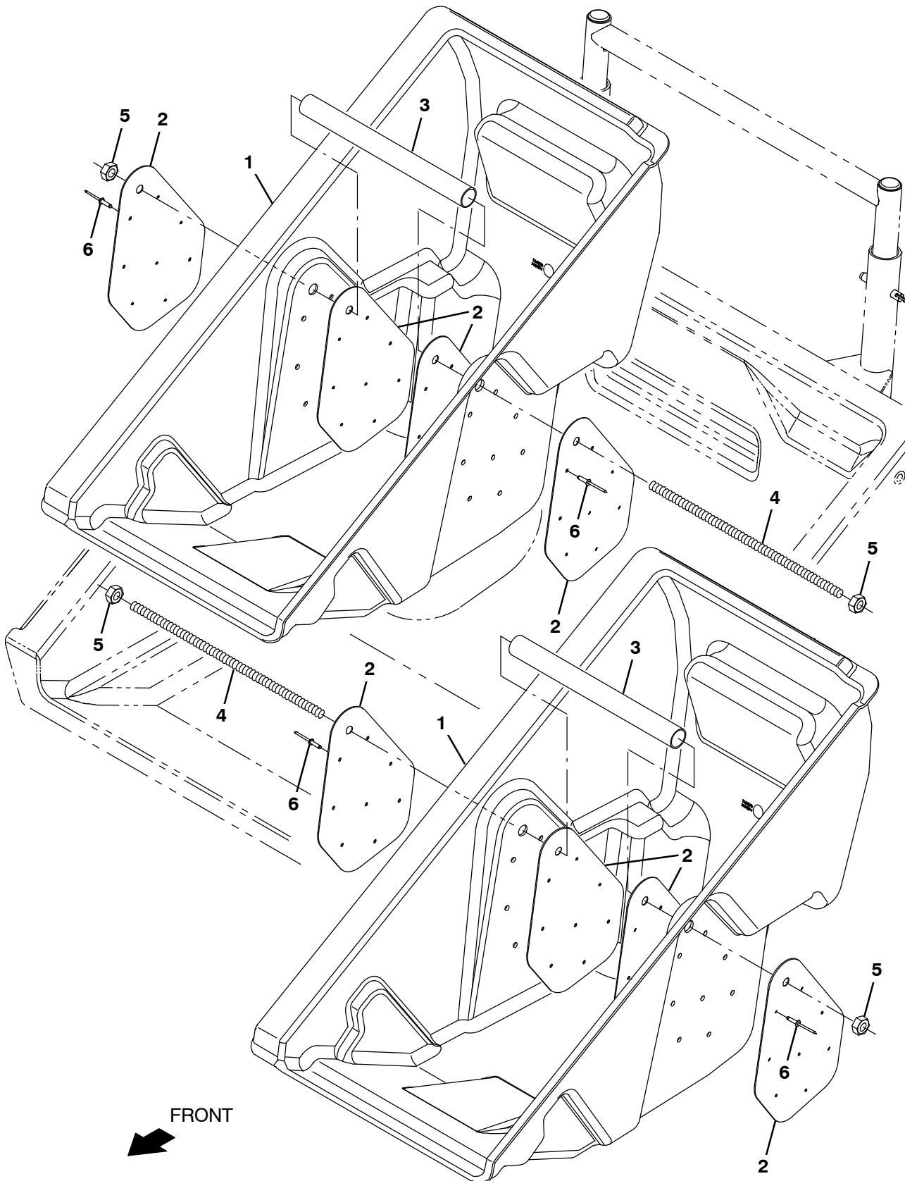
Fig. 21 – Low Dump Hopper Bins Kit
