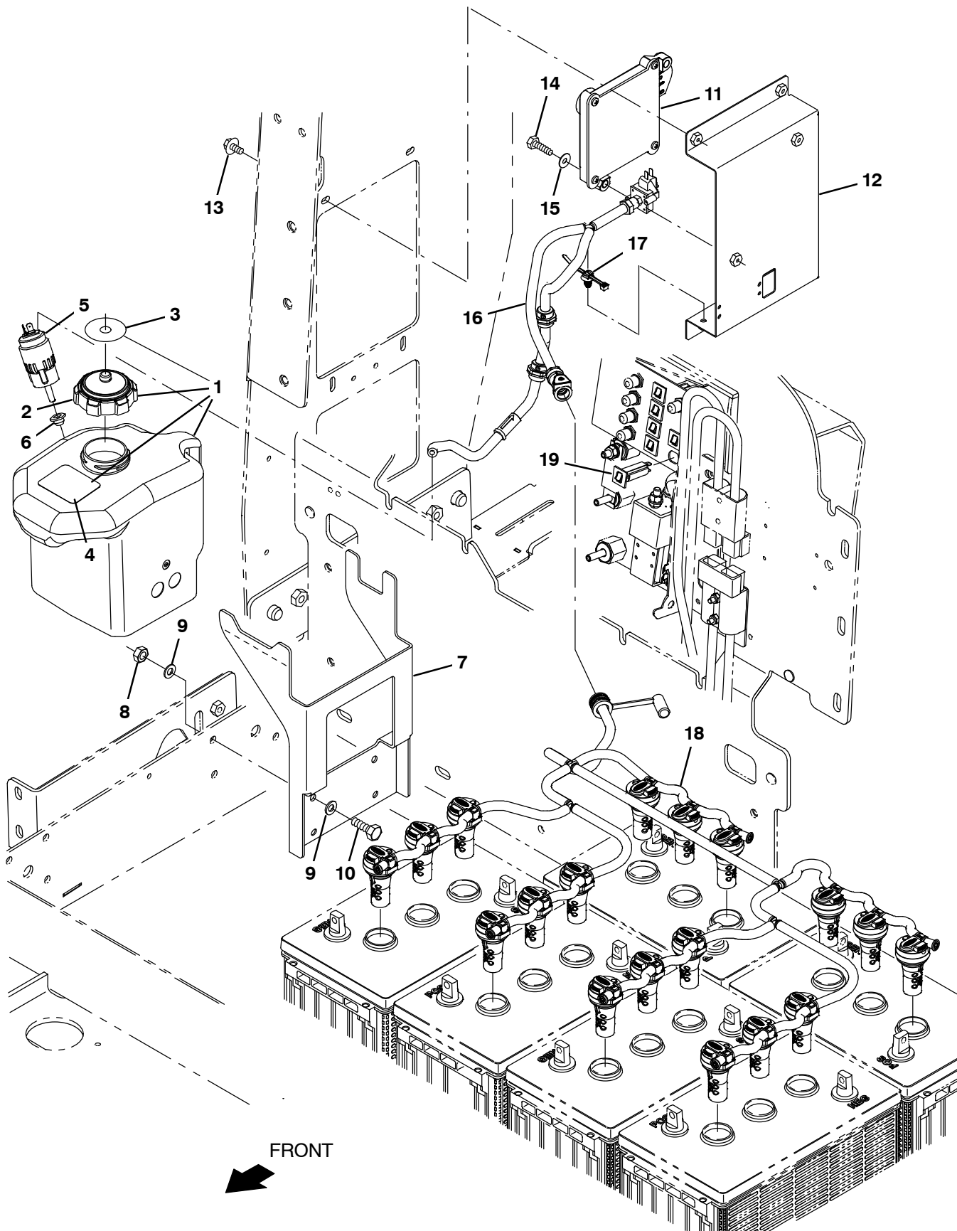
Fig. 18 – Smart-Fill Automatic Battery Watering Group
