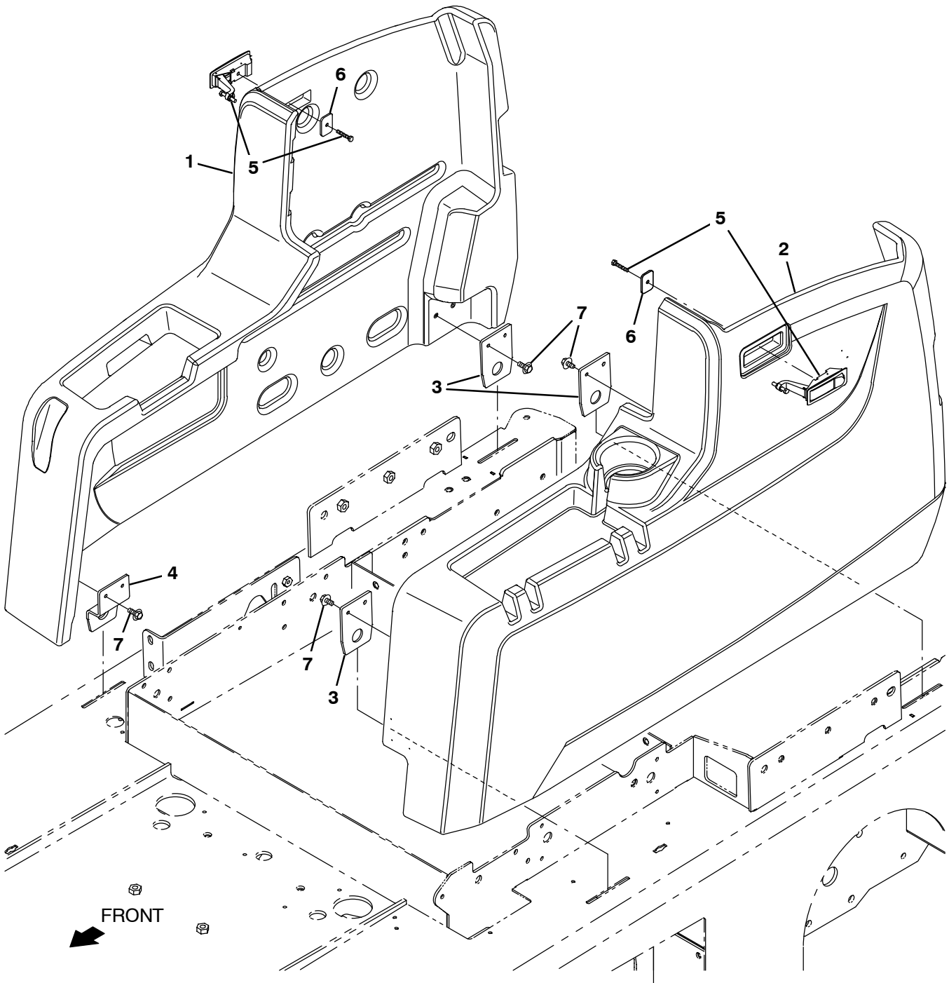
Fig. 3 – Shrouds Group
