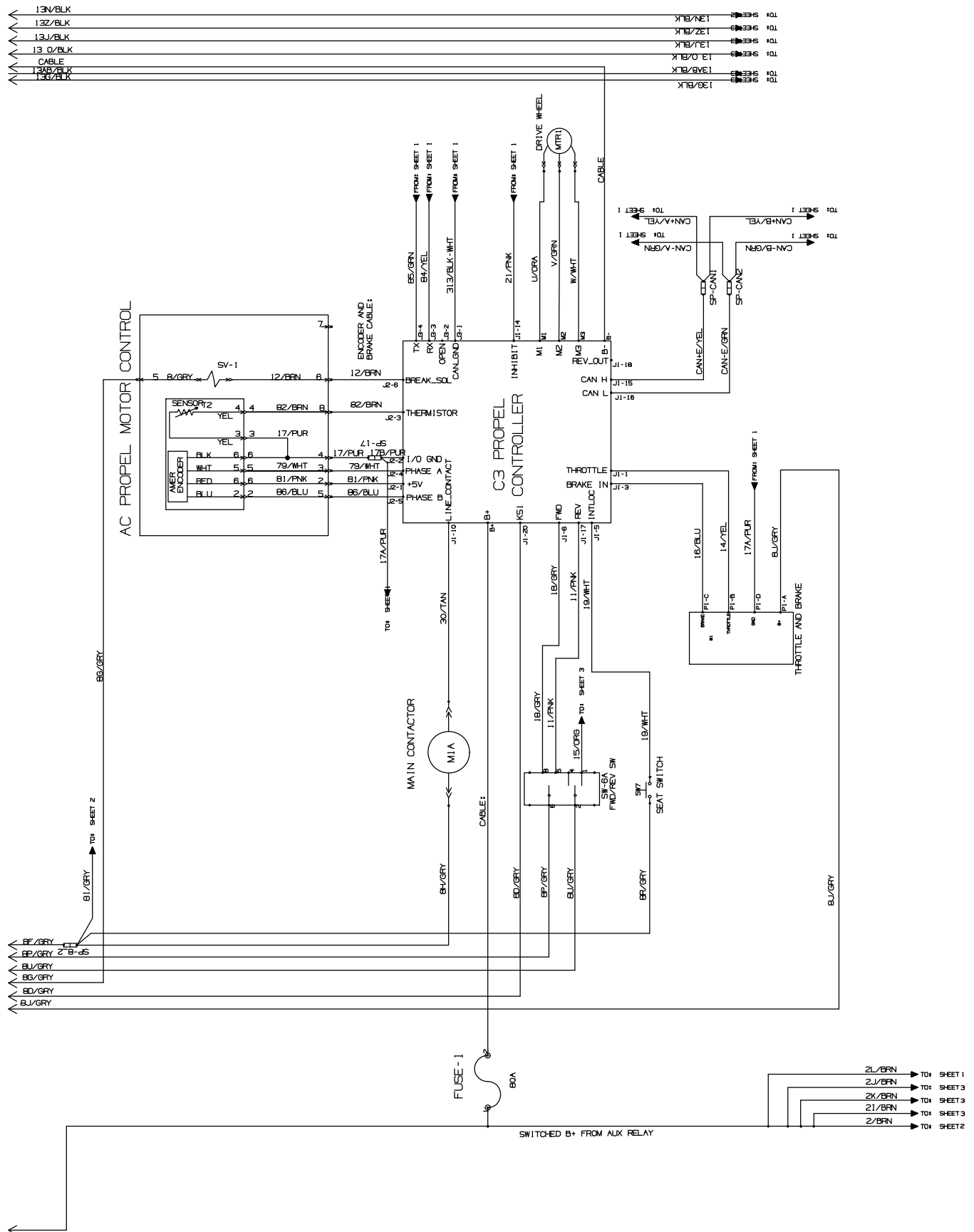
Fig. 28 – Electrical Schematic
