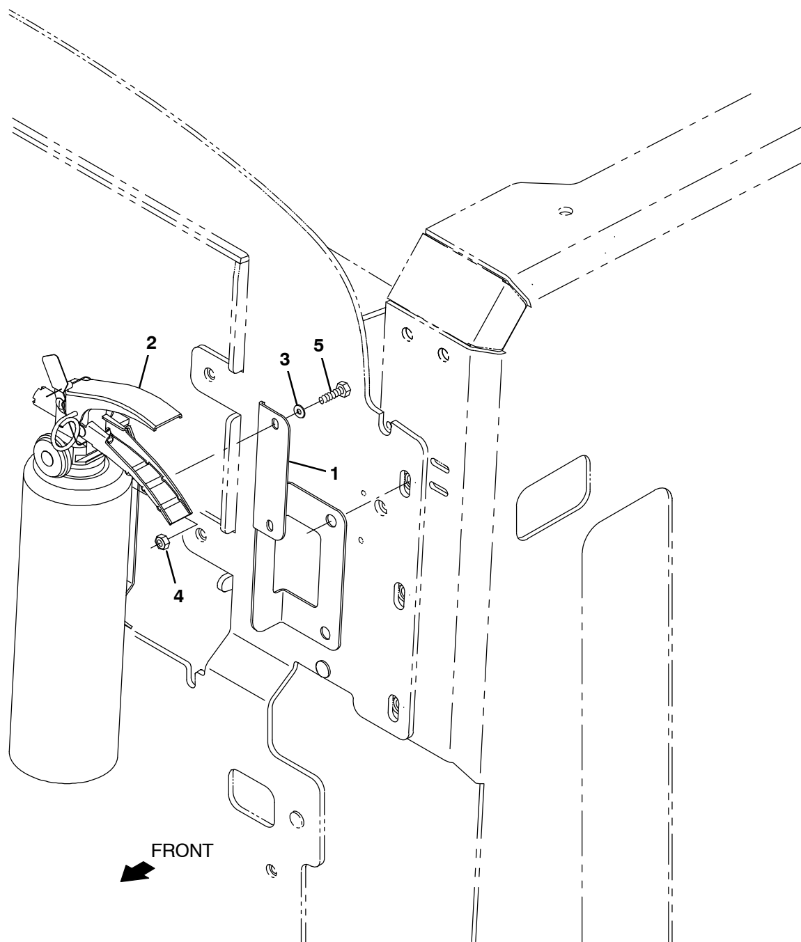
Fig. 22 – Fire Extinguisher Kit
