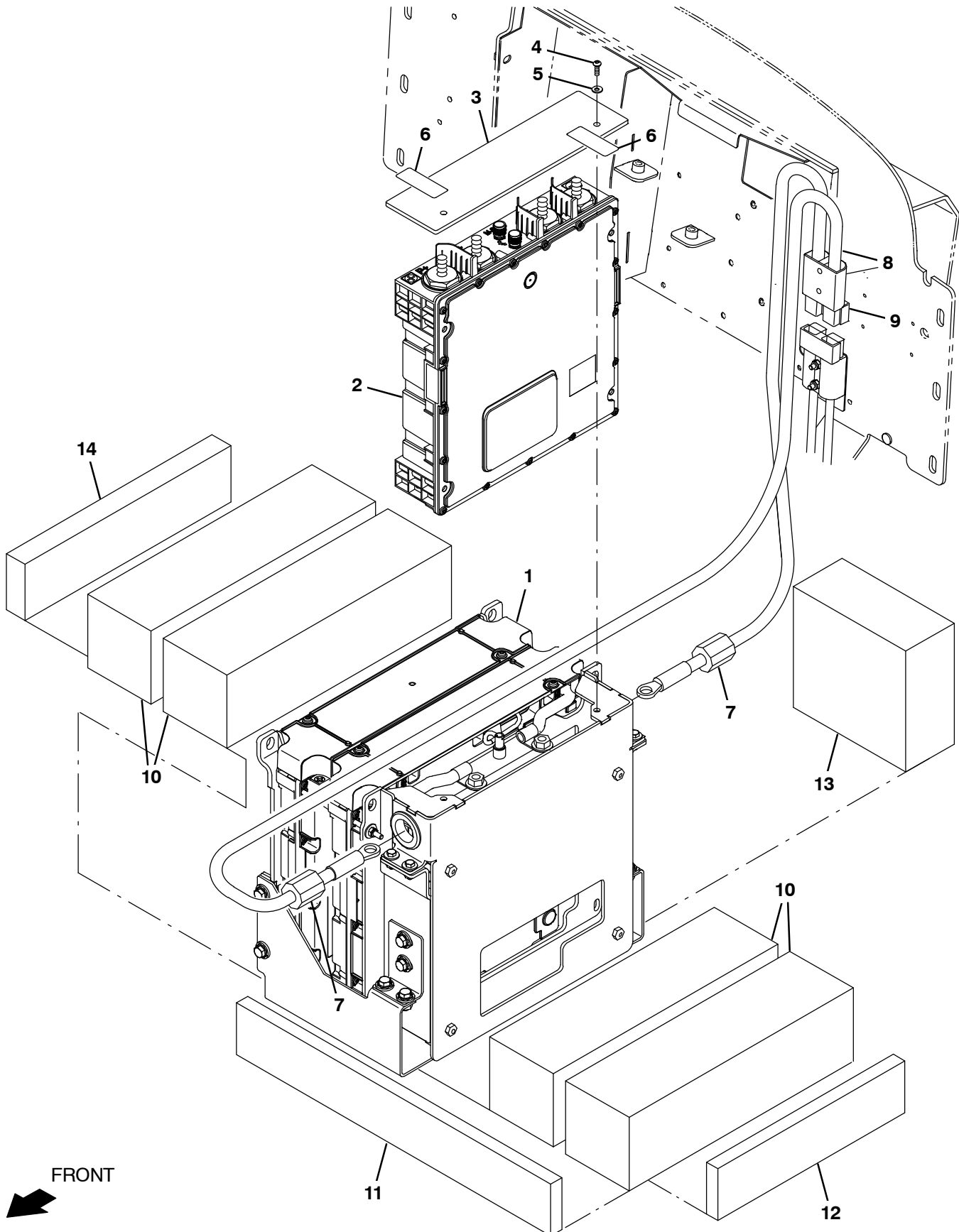
Fig. 14 – Battery Group, Lithium-Ion, 36V, 4.1 Kwh
